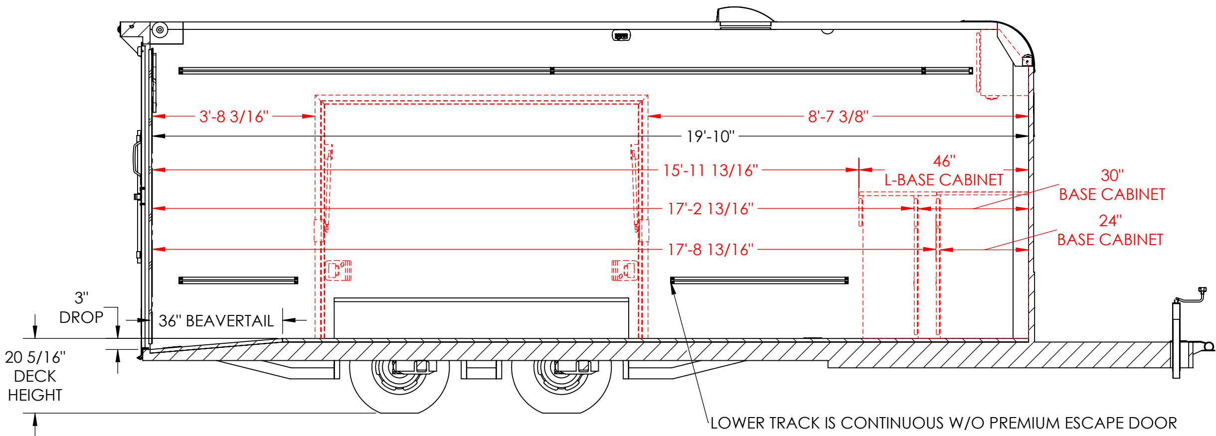
INTERIOR ROAD SIDE SECTION A-A
